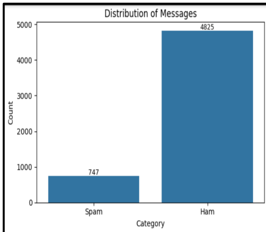
Fig 1. Distribution of Messages
