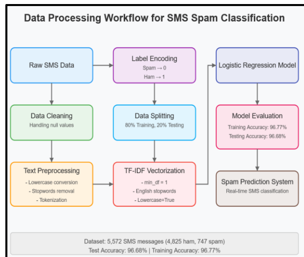
Fig 3. Spam SMS Classification - Data Processing Workflow
